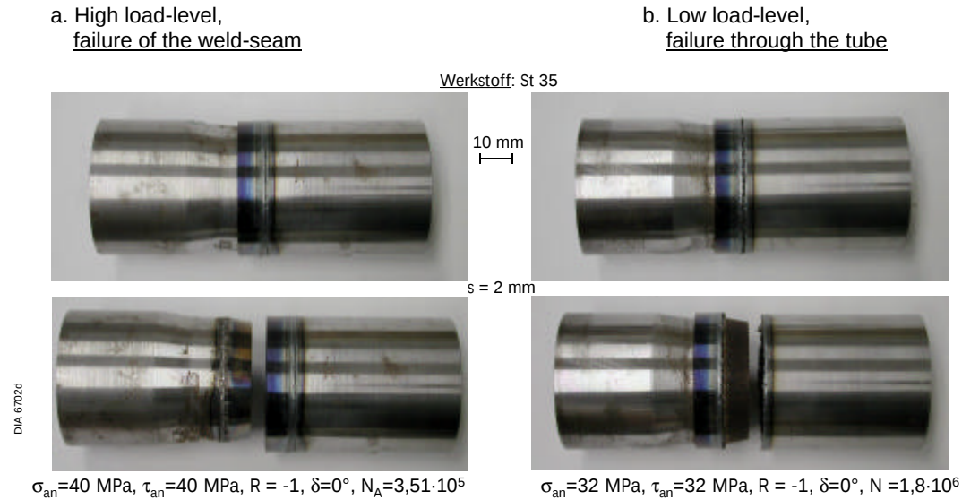
Fig. 6: Failure modes of laser beam welded tube-tube specimens
